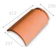
Caballete universal
