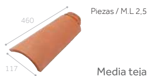
Media teja
